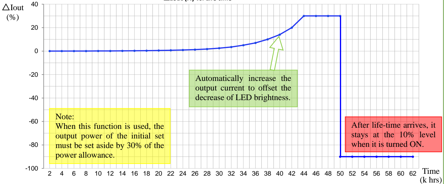
\Delta I_{out} (%) vs. Life time
