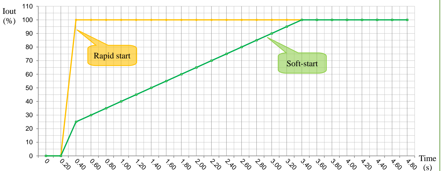
I out (%) vs. Time at Startup
